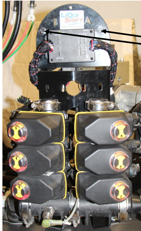
MultiTube Controller (now mounted on back of LiquiShift valve stack) Connection to A & B Manual Override Switches 14-pin to LiquiShift 2-pin (only use for sections 7-8) Manifold Controller Pressure & Flow Return B Valves A Valves
